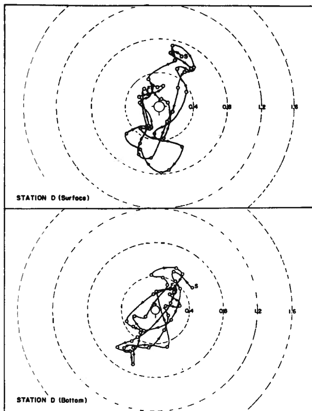
FIGURE 5. Station D hodograph of surface and bottom tidal currents.
