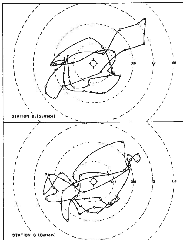
FIGURE 3. Station B hodograph of surface and bottom tidal currents.
